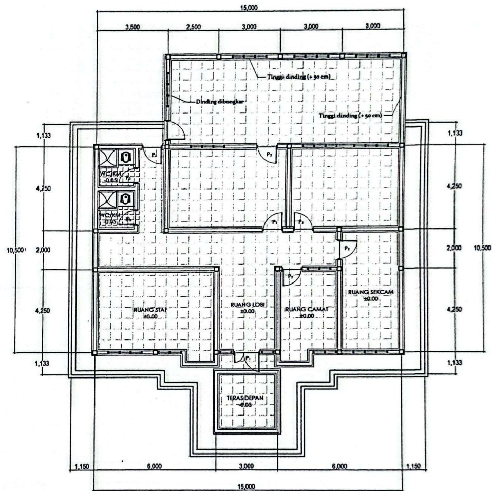
DENAH EXISTING SKALA 1 : 100
